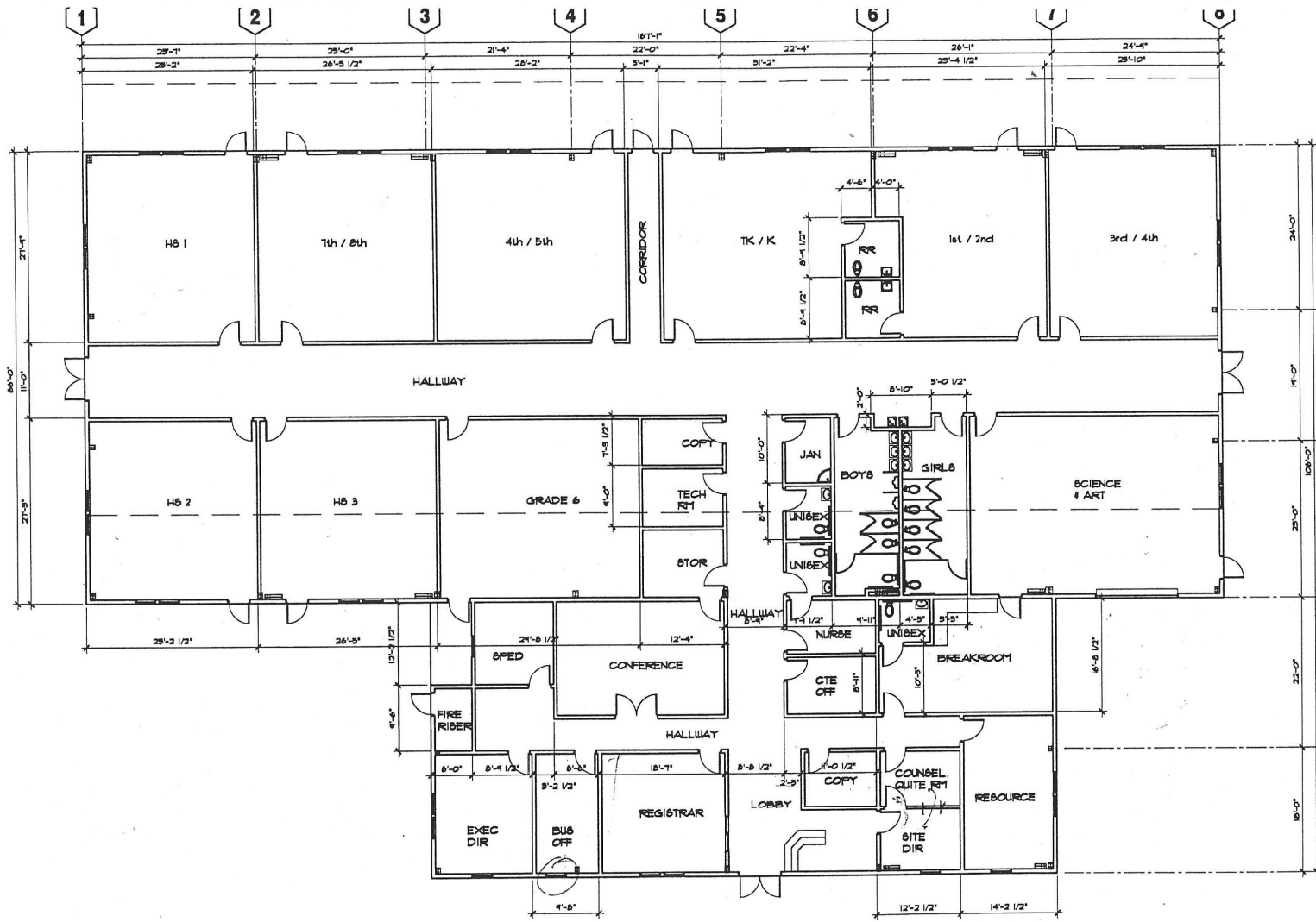
FLOOR PLAN
